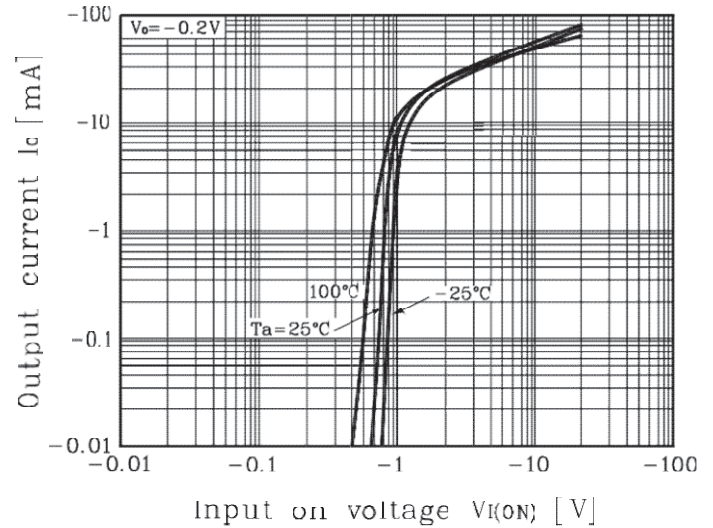
Fig. 2 I_O - V_{I(ON)}
