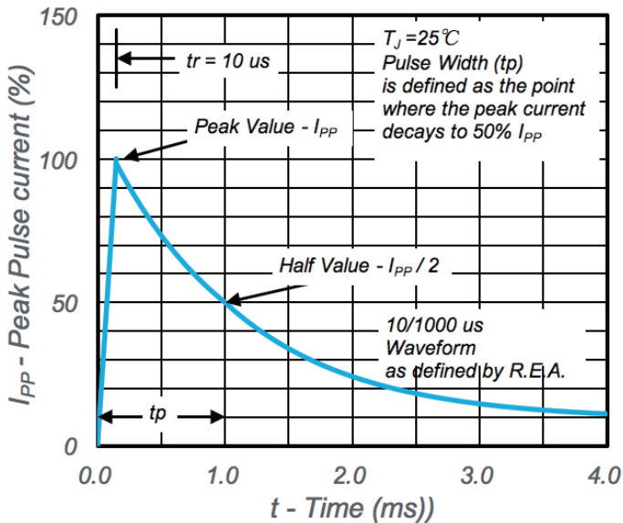
Fig.3 Pulse Waveform
