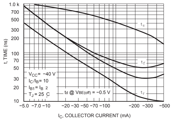
Figure 4. Switching Time
