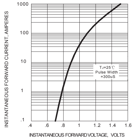
FIG.2 – TYPICAL FORWARD CHARACTERISTIC
