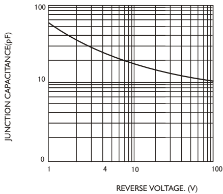
FIG.5-TYPICAL REVERSE CHARACTERISTICS
