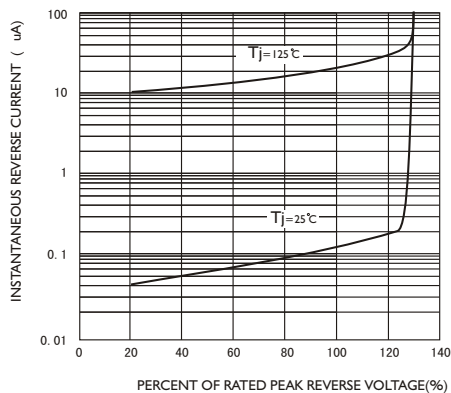
FIG.5-TYPICAL REVERSE CHARACTERISTICS
