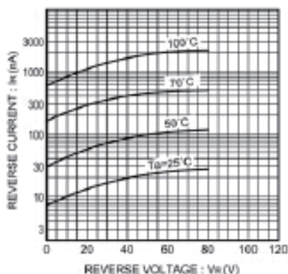
Fig. 2 Reverse characteristics
