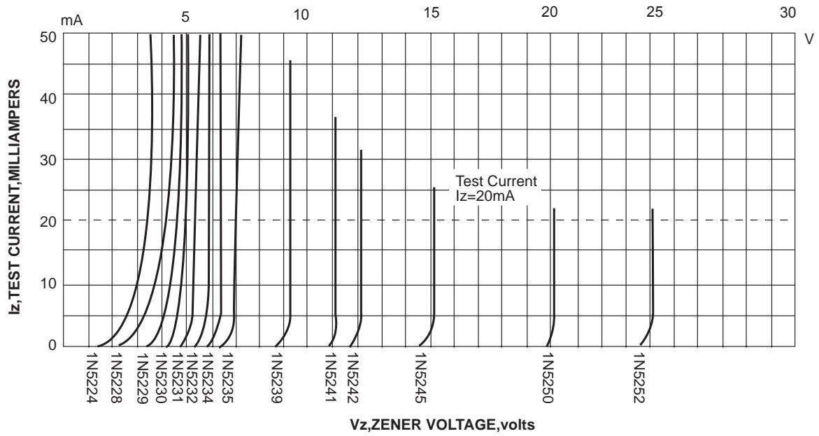
Breakdown characteristics
